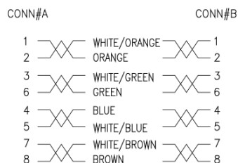
PINOUT (T658B)
